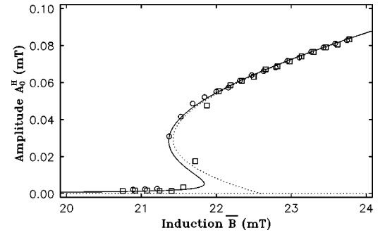
FIG. 6. Amplitude A_0^H of the stretched hexagonal pattern vs the applied magnetic induction. The open squares (circles) denote the measured amplitude under increase (decrease) of the induction, respectively. For clarity only every 10th point is shown. The solid (dotted) line give the fit by Eq. (9) with b = 1.6 \times 10^{-4} mT ( b = 0 mT), respectively. For the other parameters we obtained B_S = 22.594 mT, \gamma_1 = 7.6 mT ^{-1} , \gamma_2 = 0.9 mT ^{-1} , and g = 116.31 mT ^{-2} .
